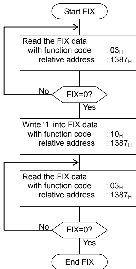
Fig.7-3 FIX procedure
